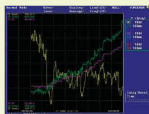
Voltage, current, and power fluctuation measurement screens
